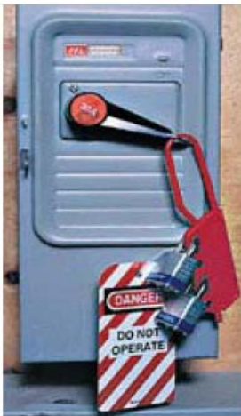
Figure 5: Locking off methods incorporating danger tags
