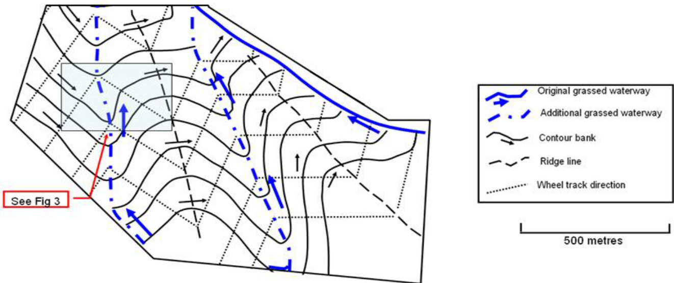
Figure 2 A CTF layout with two herringbone patterns
